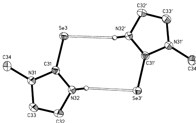
Figure 8. Molecular structure of (\text{seim}^{\text{Me}})\text{H} . Selected bond lengths (Å): C(11)–Se(1) 1.849(3), C(21)–Se(2) 1.849(3), C(31)–Se(3) 1.849(3), Se(1)⋯N(22) 3.414(3), Se(2)⋯N(12) 3.390(3), Se(3)⋯N(32') 3.394(3).
