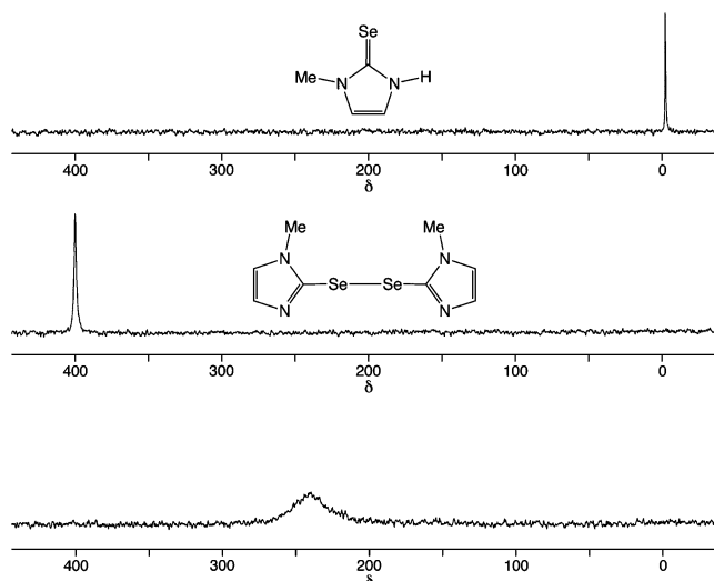
Figure 9. ^{77}\text{Se} NMR spectra of ( \text{seim}^{\text{Me}}\text{H} ) (top), ( \text{seim}^{\text{Me}}_2 ) (middle), and a 1.3:1 mixture (bottom), corresponding to an exchange rate of \sim 25,000 \text{ s}^{-1} .
